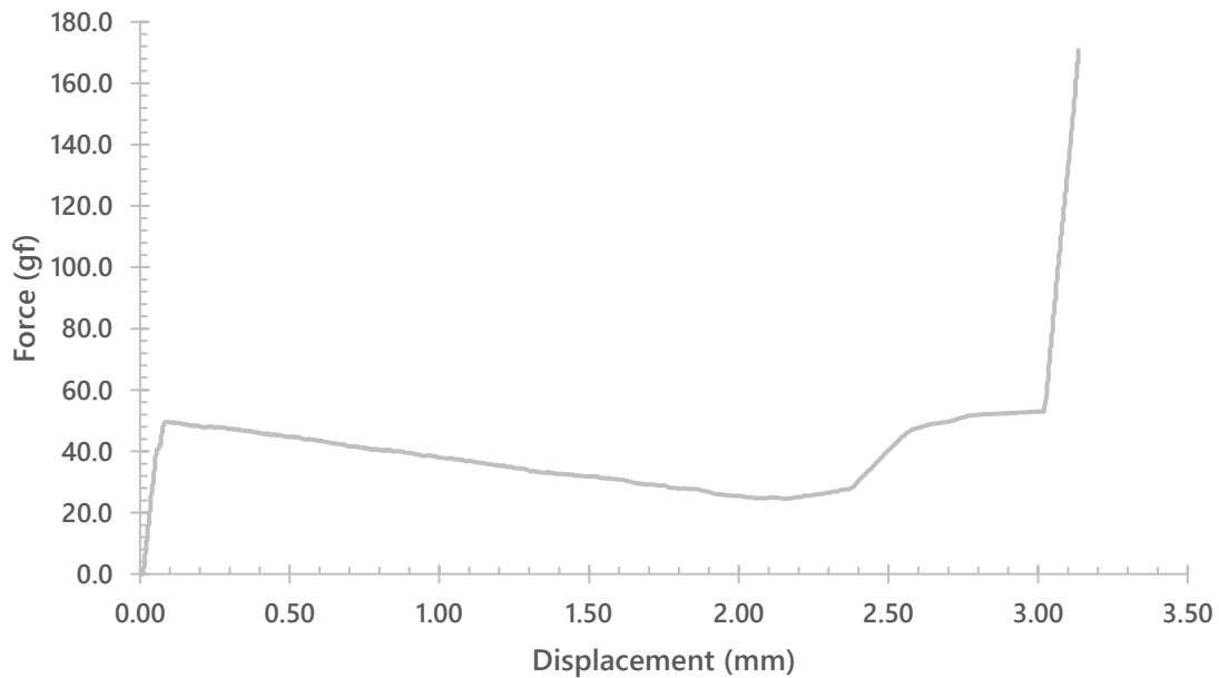
Wingtree BM11 (Upstroke)
